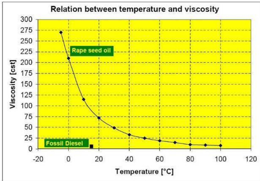
Viscosity of cold pressed rape seed oil as function of temperature
