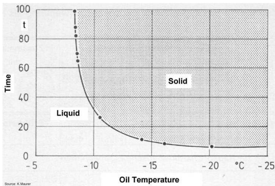
Liquid/solid phase diagram for cold pressed rape seed oil as a function oil temperature and time in hours.
